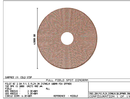
Figure 8. Cold stop surface, showing light-loss due to imperfect re-imaging of the pupil.
