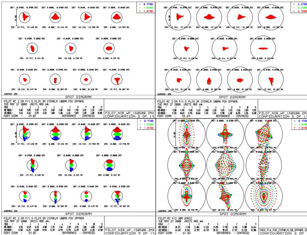
Figure 9. NIR image quality for (in order) Y and K_{\text{dark}} -band wide-field use at zenith; Y-band use at ZD=70°; Y-band use with the Barlow lenses. Airy disc and 2 pixel scale bar is shown in each case.
