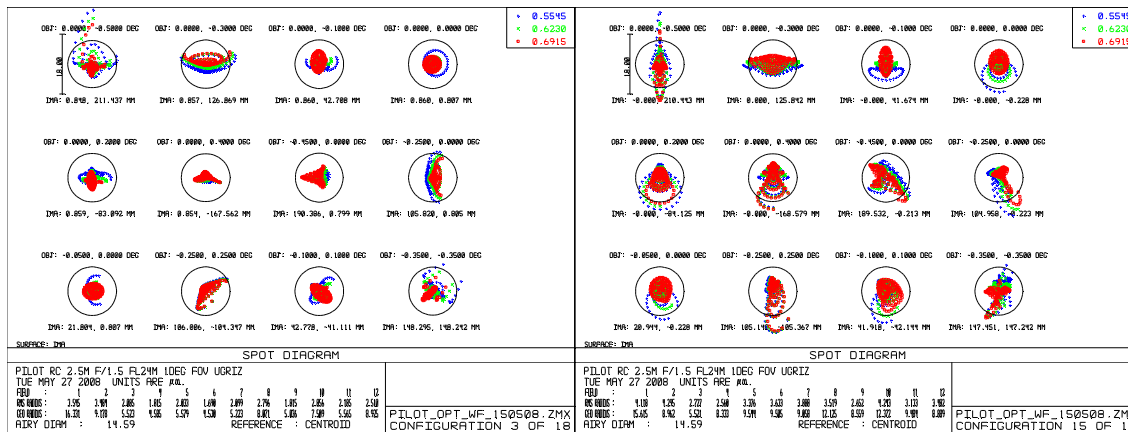
Figure 4. r-band spot diagrams at zenith and ZD=70^\circ , showing the Airy disc.
