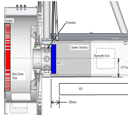
Figure 3. Proposed ADC location on wide-field optical camera
