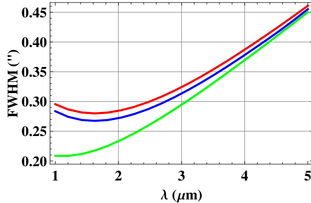
Figure 12. NIR Image quality for wide-field (red) or narrow-field (blue) use in median conditions, and for narrow-field use when the boundary layer is entirely below 30m (green).
