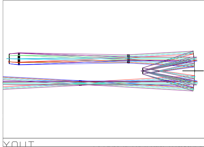
Figure 10 NIR camera optical design for diffraction-limited use at zYJHK . Not shown are the 4 fold mirrors required to keep the overall path length and detector placement the same as for wide-field use.
