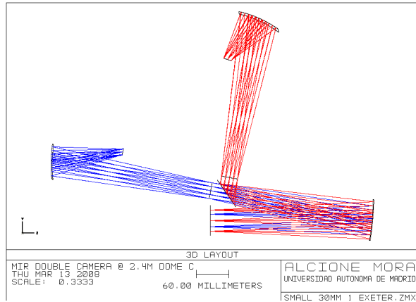
Figure 13. Mid-IR camera-spectrograph optical design
